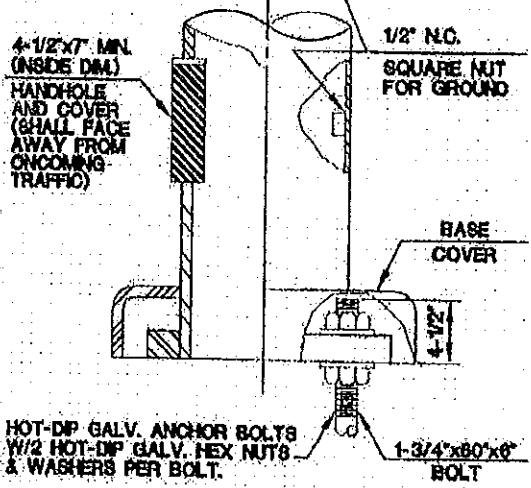
POLE MOUNTING DETAIL
