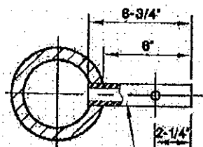
2" SCH. 40 PIPE TENON WITH 7/16" THRU HOLE FOR ELEVATOR PLUMBIZER DETAIL A-A
