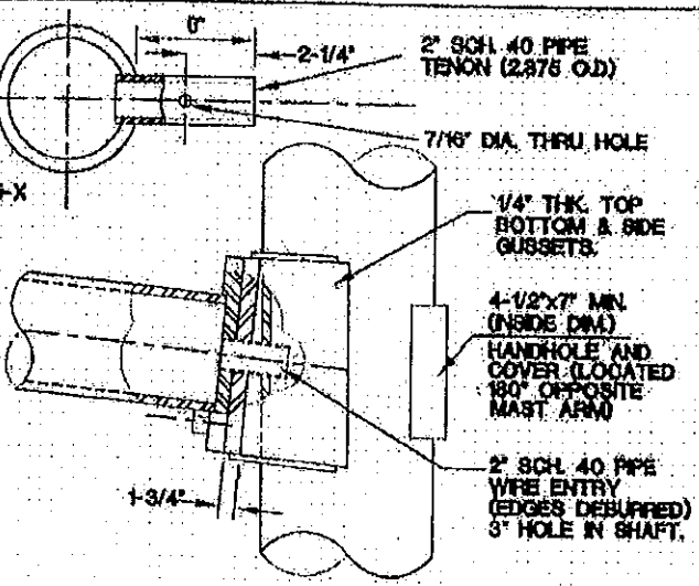
POLE MOUNTING DETAIL
